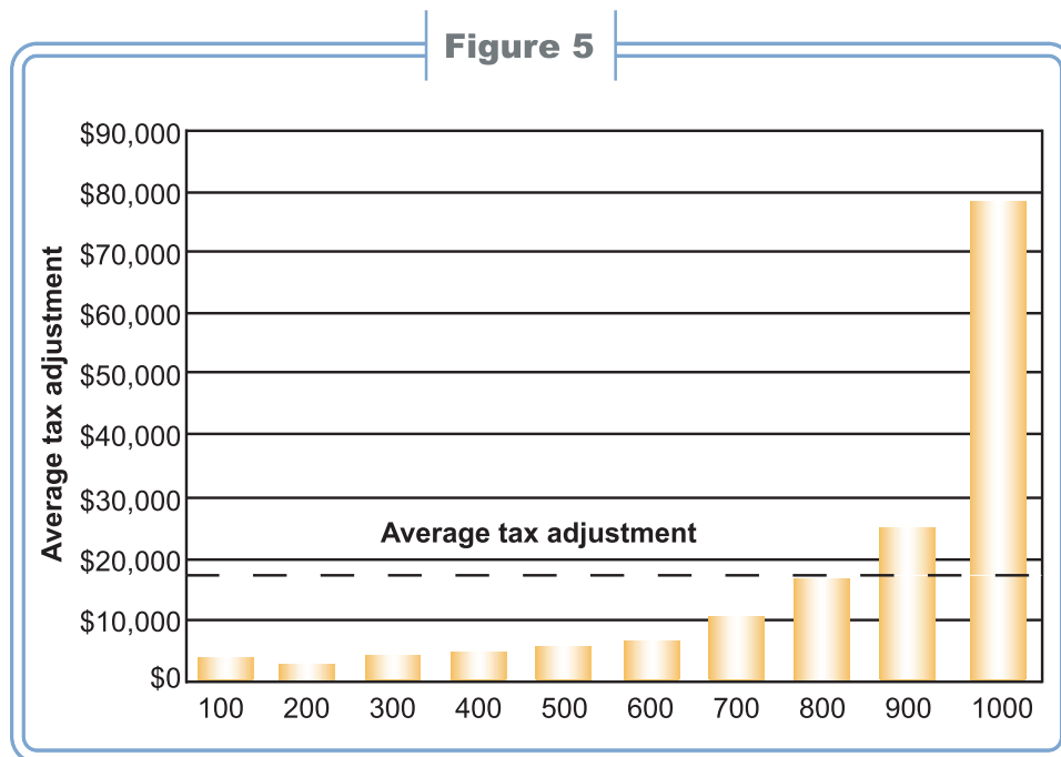
Figure 5: Average final adjustment by score for sales tax audits performed between 1996 and 2002
